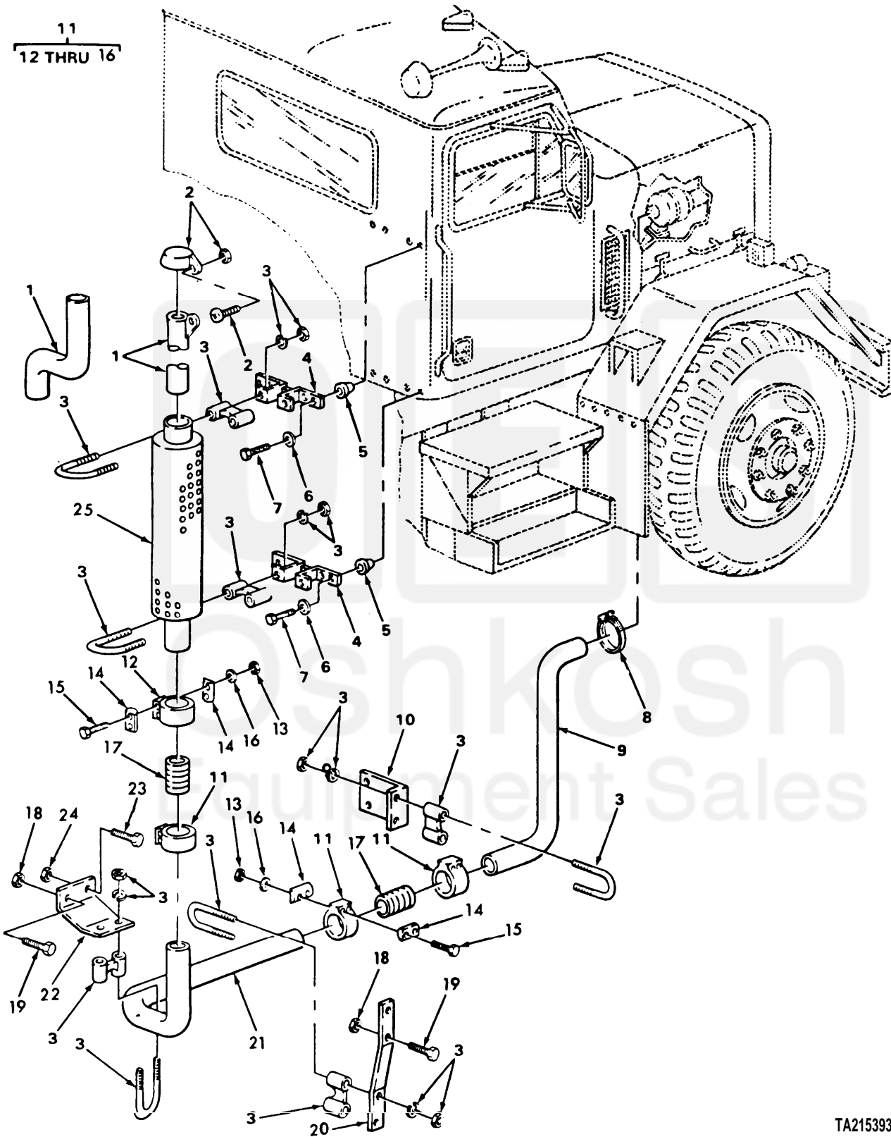
FIGURE 18. EXHAUST SYSTEM.
